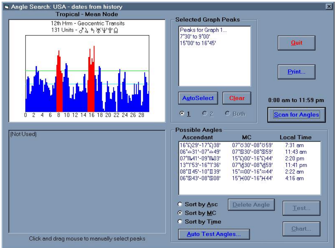
Figure 1 -Geocentric Graph of USA Dates Jigsaw 2
