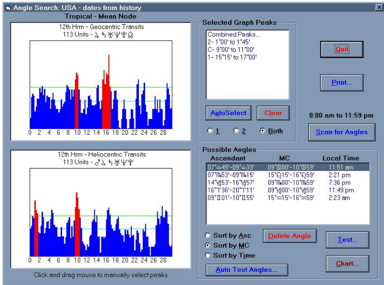
Figure 2 -Geocentric and Heliocentric Graphs compared for USA Dates Jigsaw 2
